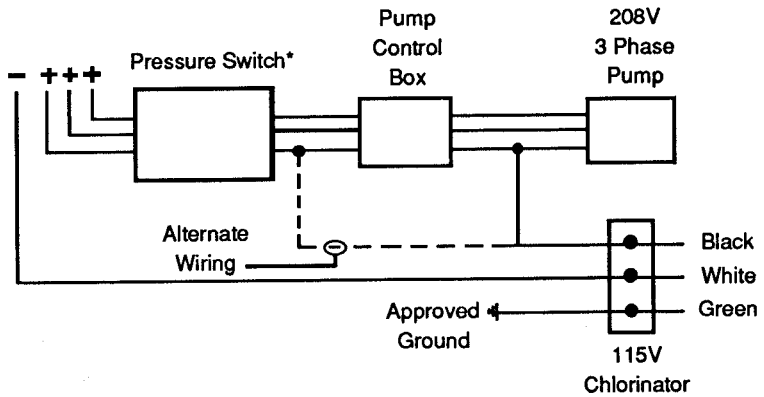
Wiring Diagram 115V Chlorinator 208V Well Pump
