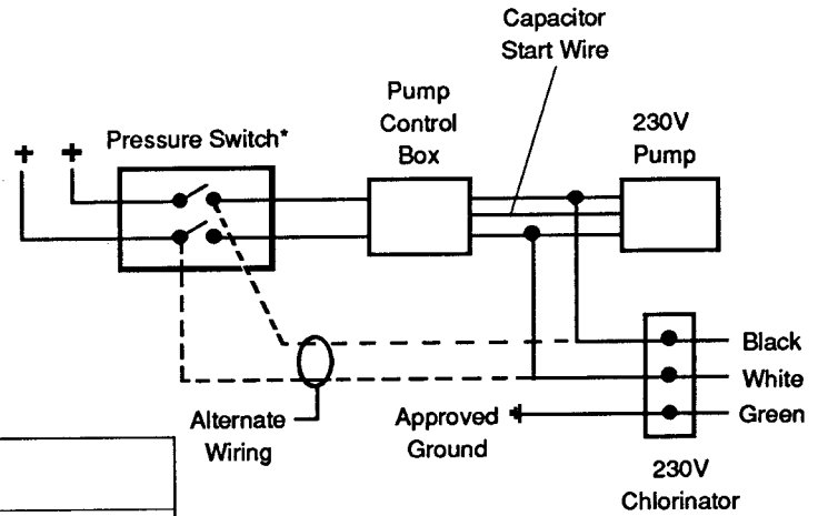
Wiring Diagram 230V Chlorinator 230V Well Pump
